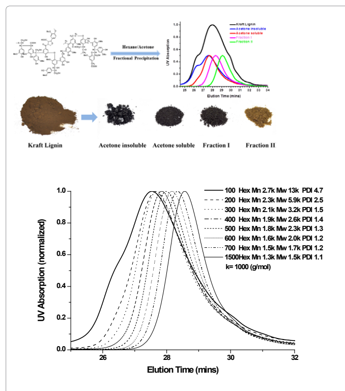
Figure 1: Normalized and superimposed GPC chromatograms of kraftlignin fractions origination from a fine fractional precipitation procedure afforded by the addition of incremental amounts of hexanes (Hex) into acetone solutions of the lignin.
